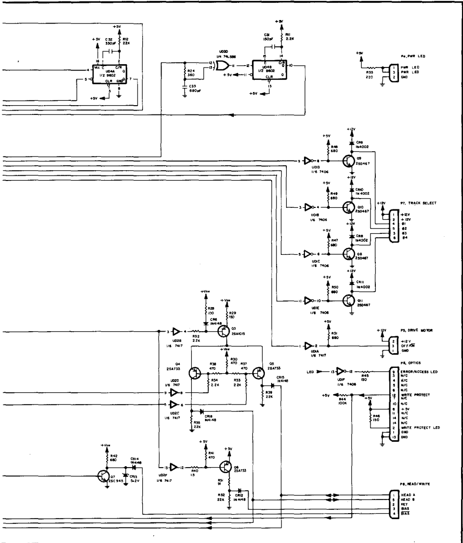
schematic, Model 1542 (cont.)
